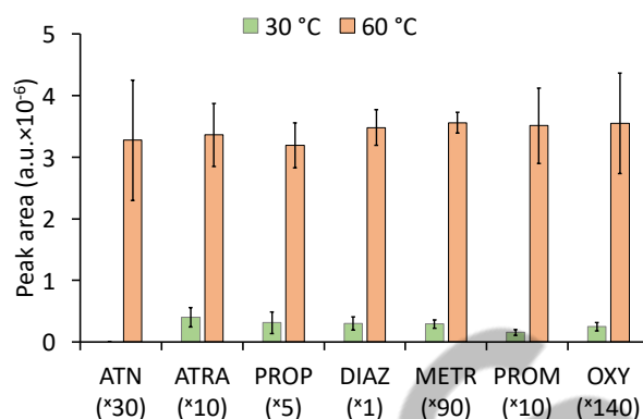
Figure 4 – Effect of extraction temperature on responses of analytes
